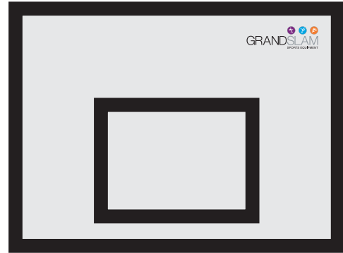
Half size 1200 x 900mm BB830, BB836
