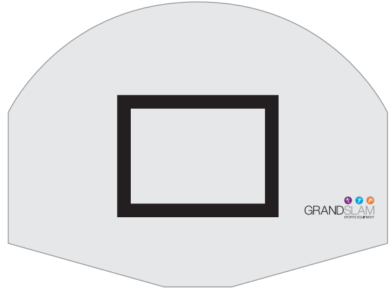
Three-quarter size fan-shaped 1400 x 1050mm BB845
